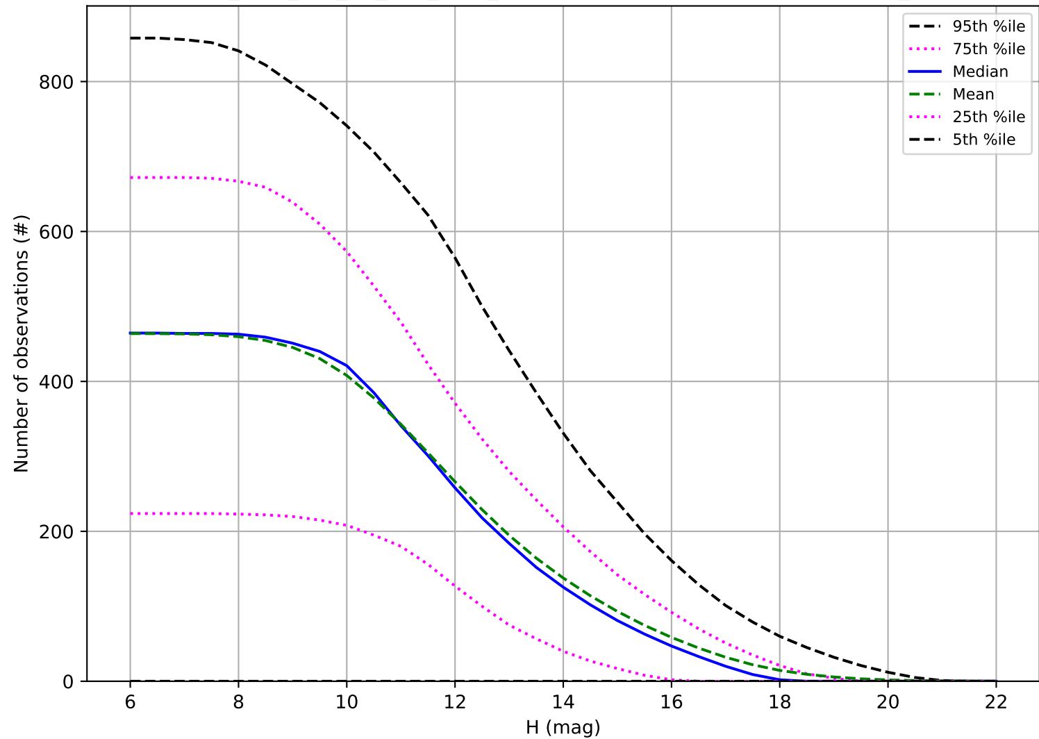
too_elab_r16_d2_griz_v3.4_10yrs: Number of observations OCC_r5
