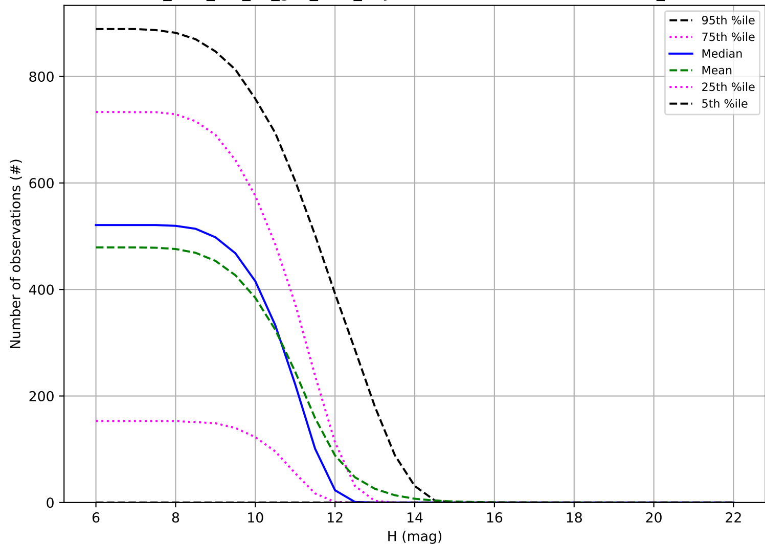
too_elab_r16_d2_griz_v3.4_10yrs: Number of observations OCC_r20
