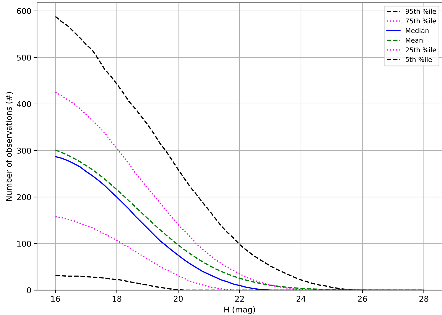
too_elab_r16_d2_griz_v3.4_10yrs: Number of observations NEO
