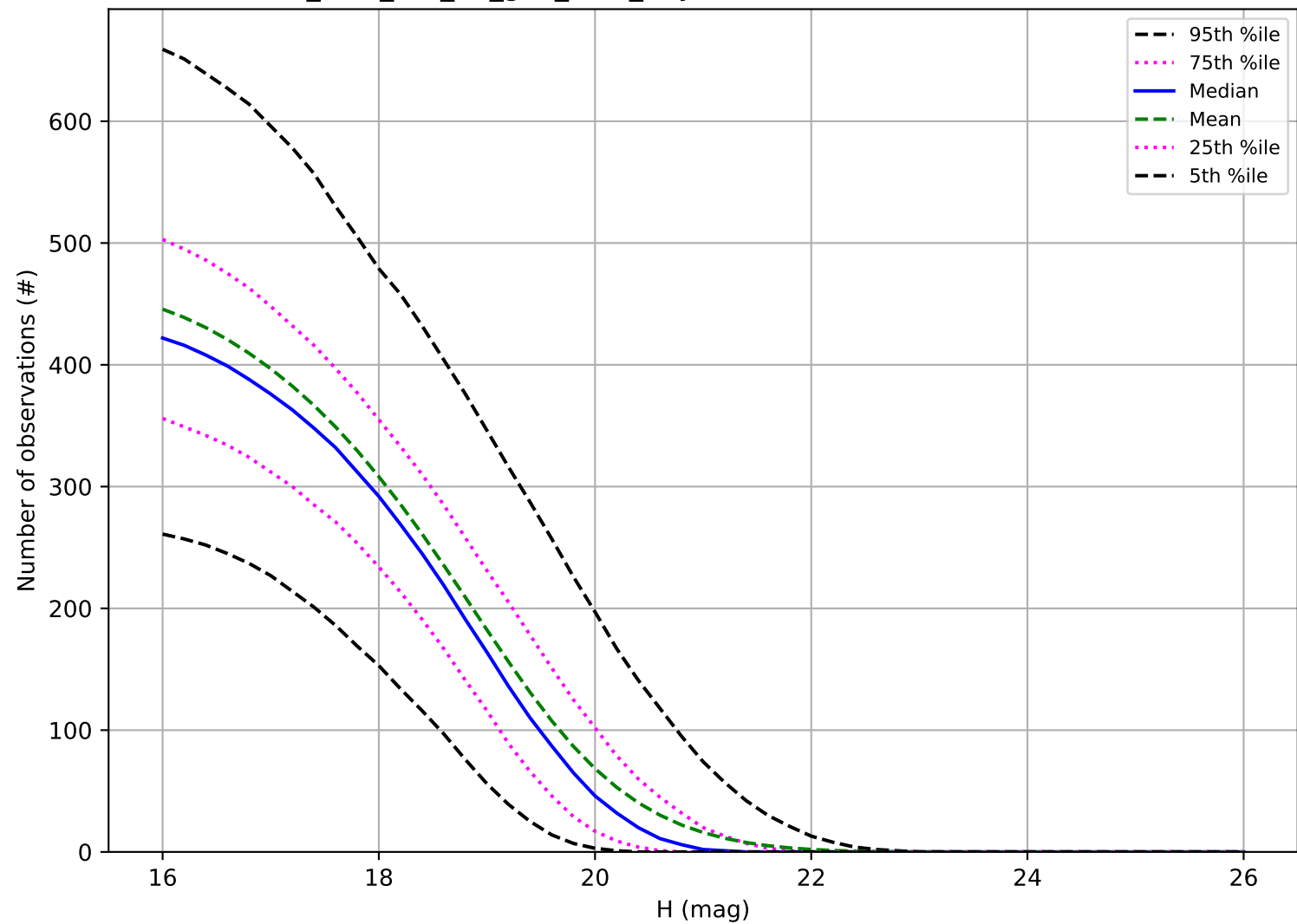
too_elab_r16_d2_griz_v3.4_10yrs: Number of observations MBA
