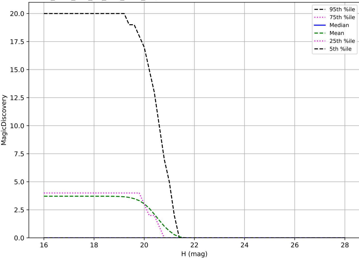
too_elab_r16_d2_griz_v3.4_10yrs: Vaira 6 detections in 60 nights detection loss
