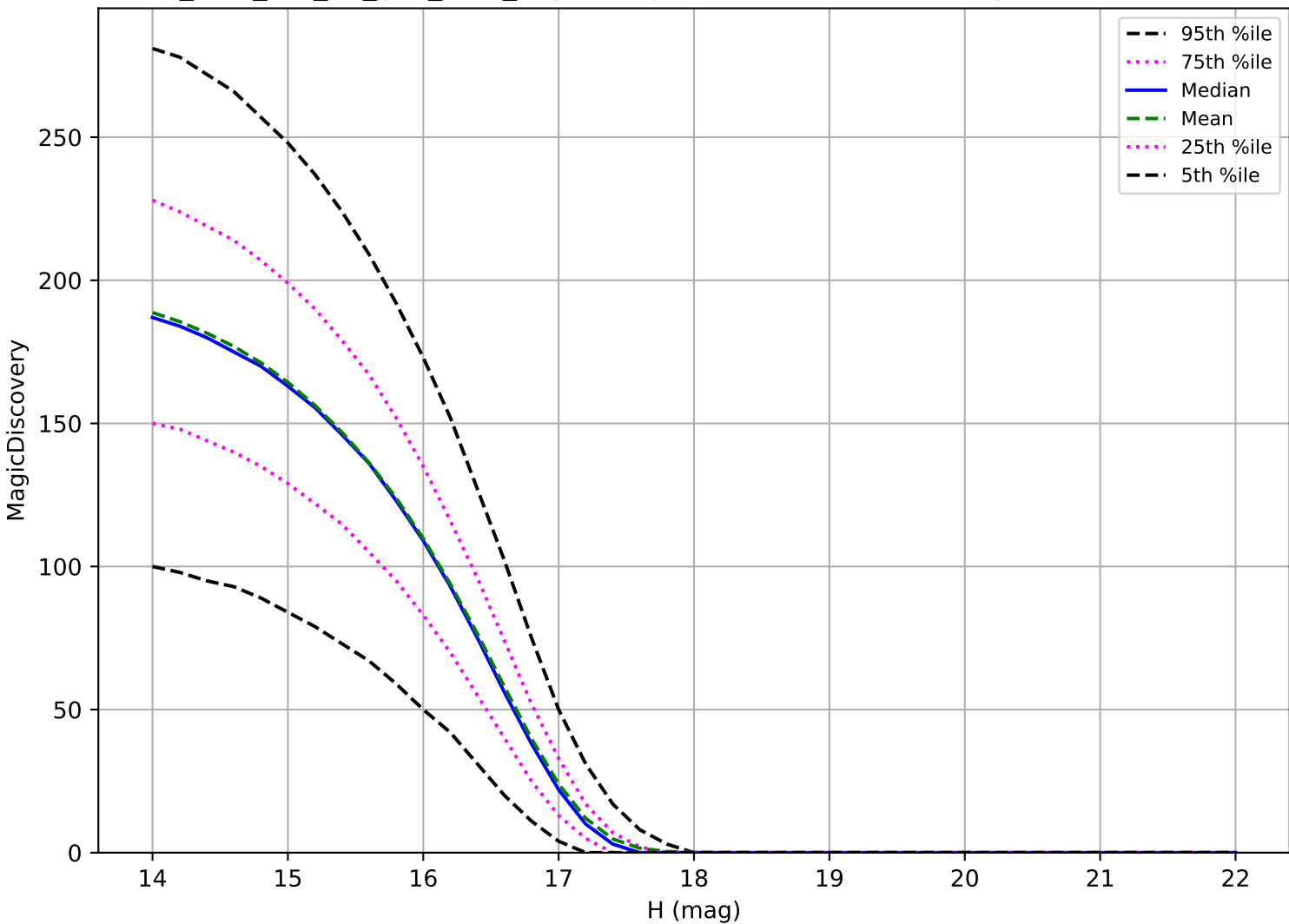
too_elab_r16_d2_griz_v3.4_10yrs: Trojan 6 detections in 60 nights detection loss
