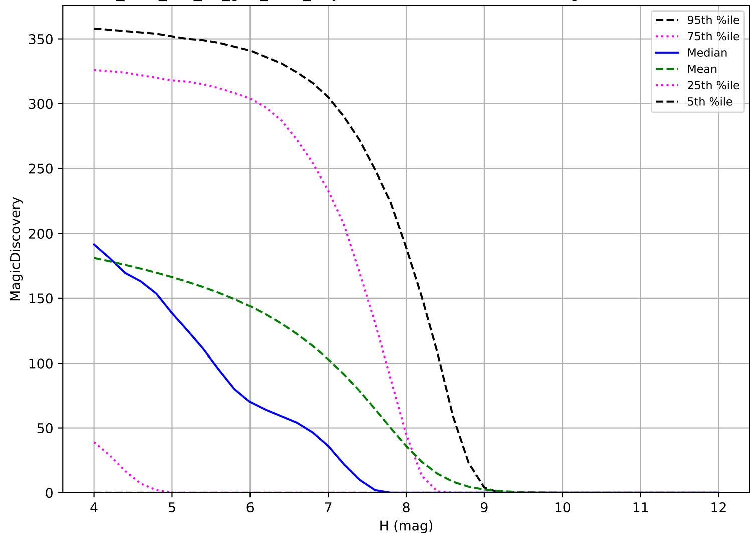
too_elab_r16_d2_griz_v3.4_10yrs: TNO 6 detections in 60 nights detection loss
