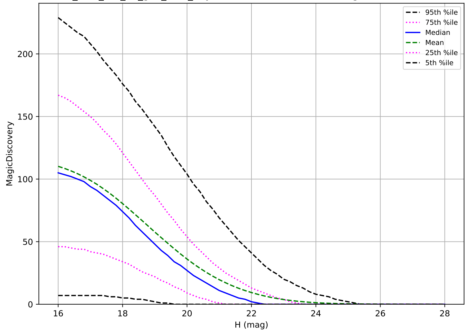
too_elab_r16_d2_griz_v3.4_10yrs: PHA 6 detections in 60 nights detection loss
