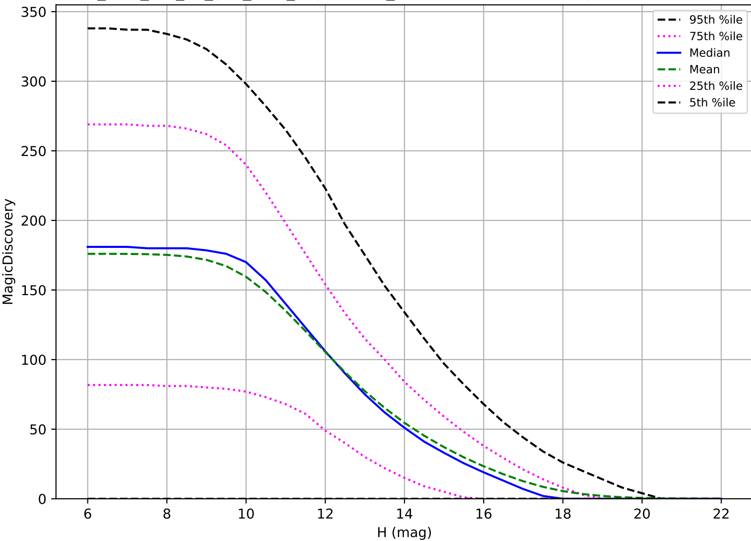
too_elab_r16_d2_griz_v3.4_10yrs: OCC_r5 6 detections in 60 nights detection loss
