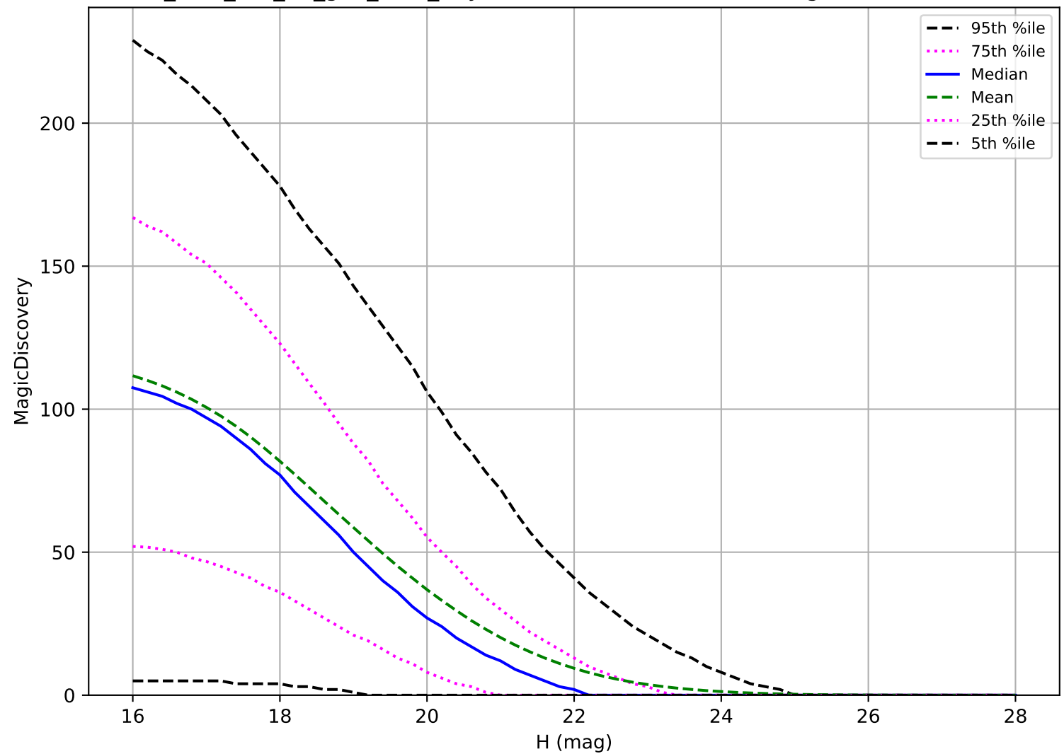
too_elab_r16_d2_griz_v3.4_10yrs: NEO 6 detections in 60 nights detection loss
