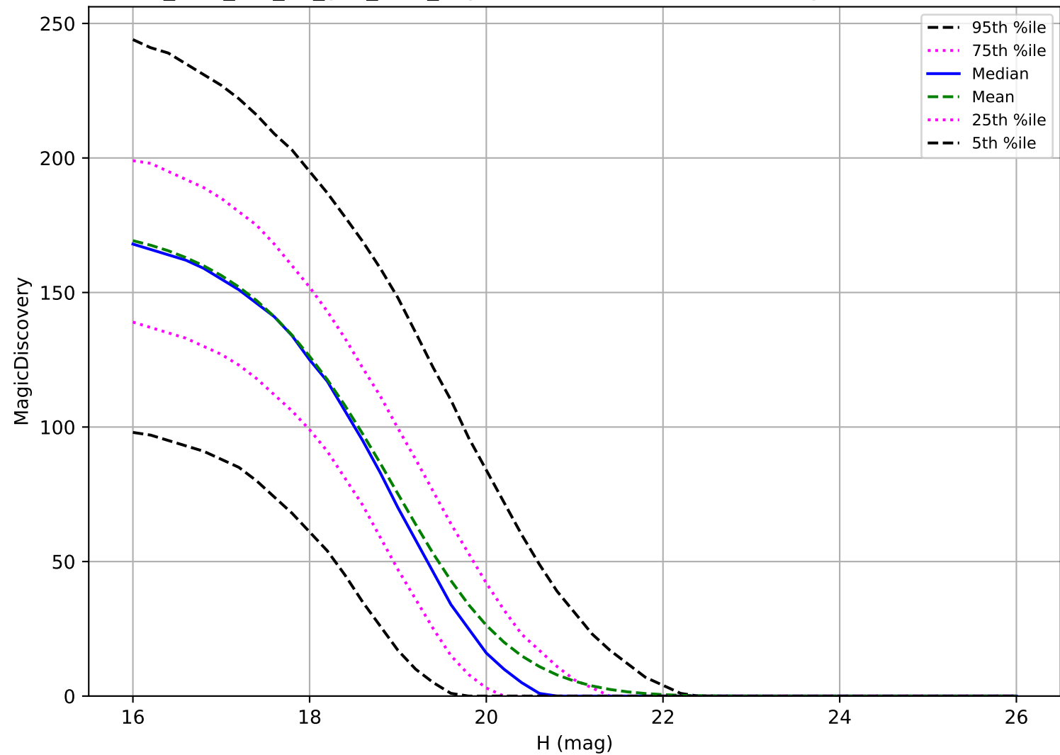
too_elab_r16_d2_griz_v3.4_10yrs: MBA 6 detections in 60 nights detection loss
