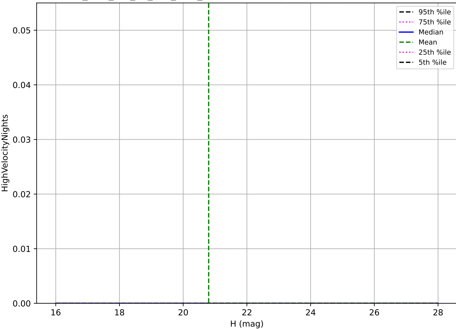
too_elab_r16_d2_griz_v3.4_10yrs: Vatira High velocity pair detection loss
