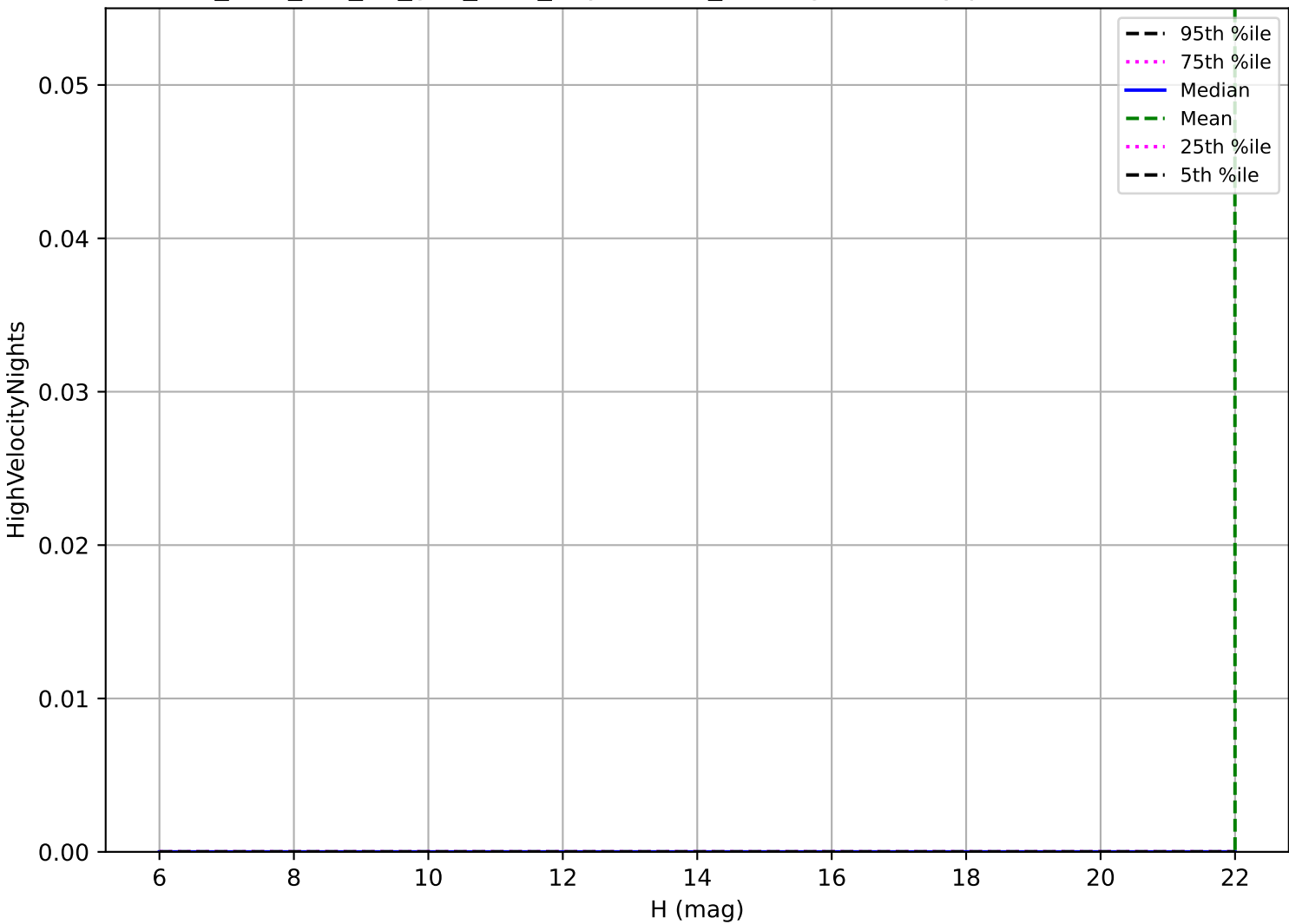
too_elab_r16_d2_griz_v3.4_10yrs: OCC_r20 High velocity pair detection loss
