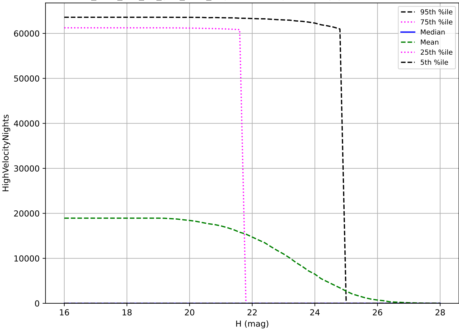
too_elab_r16_d2_griz_v3.4_10yrs: NEO High velocity pair detection loss
