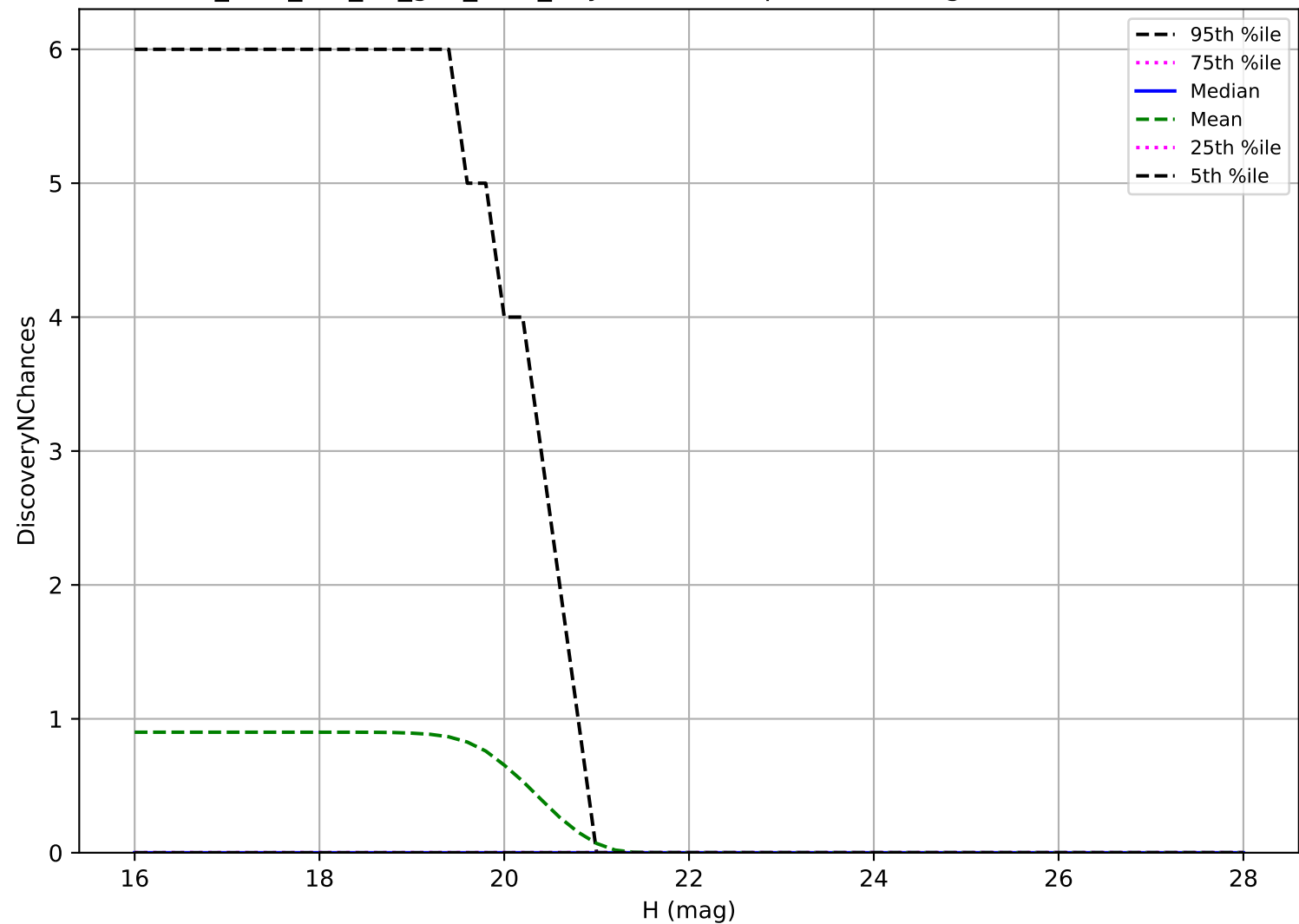
too_elab_r16_d2_griz_v3.4_10yrs: Vatira 3 pairs in 15 nights detection loss
