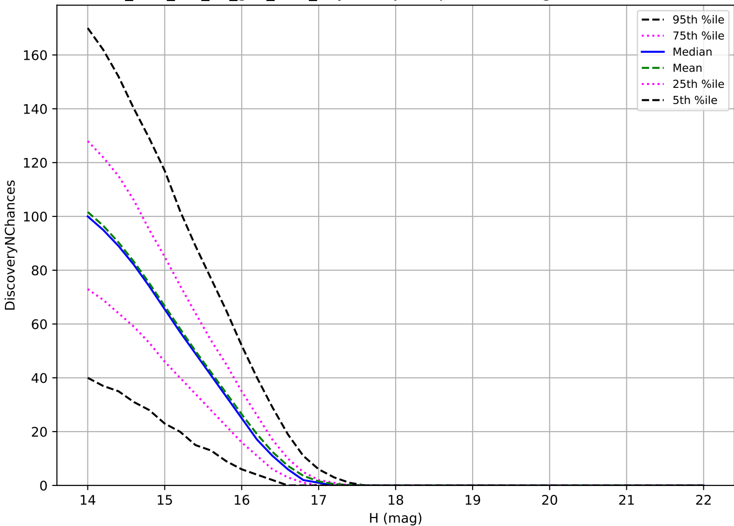
too_elab_r16_d2_griz_v3.4_10yrs: Trojan 3 pairs in 15 nights detection loss
