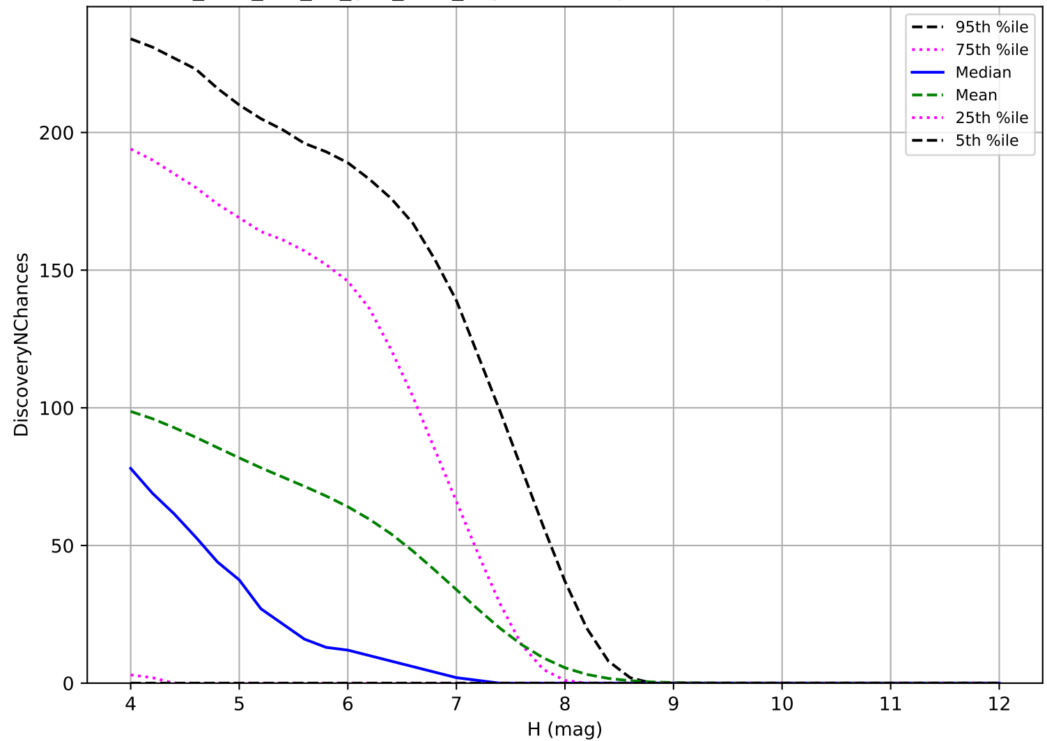
too_elab_r16_d2_griz_v3.4_10yrs: TNO 3 pairs in 15 nights detection loss
