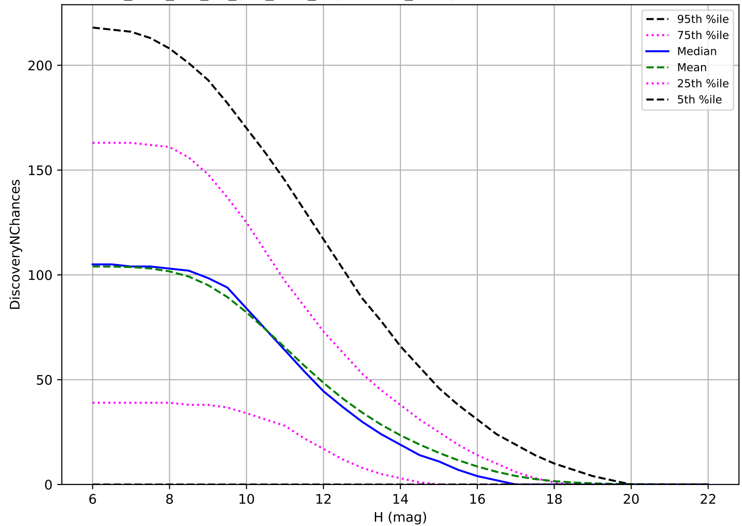
too_elab_r16_d2_griz_v3.4_10yrs: OCC_r5 3 pairs in 15 nights detection loss
