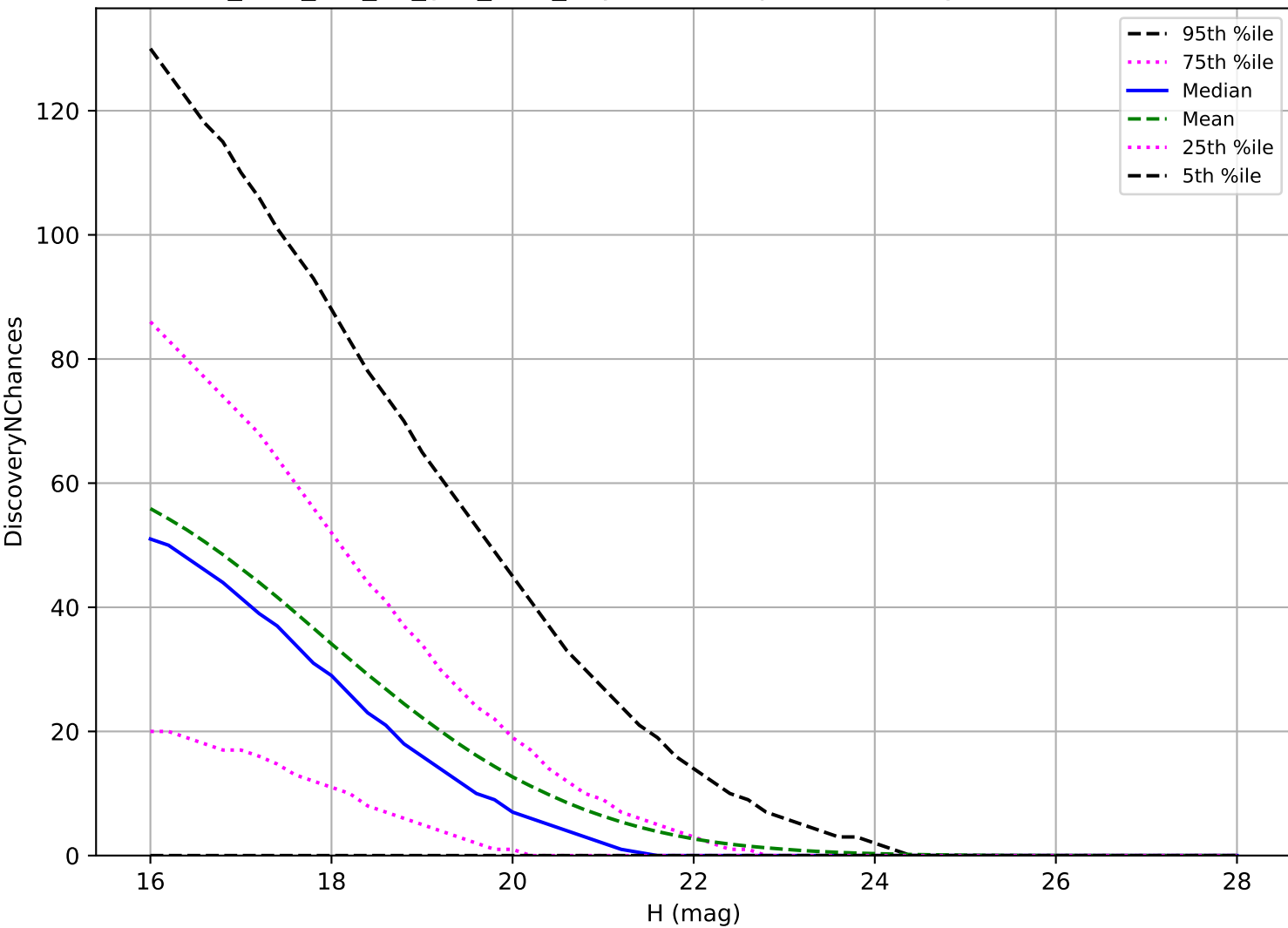
too_elab_r16_d2_griz_v3.4_10yrs: NEO 3 pairs in 15 nights detection loss
