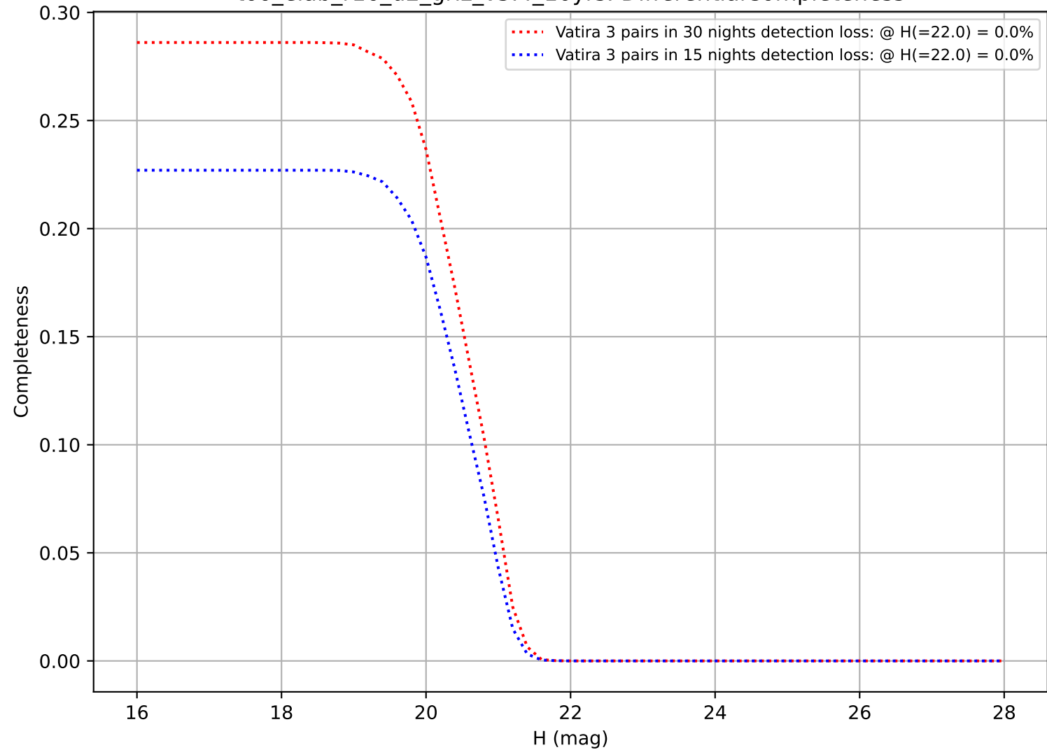
too_elab_r16_d2_griz_v3.4_10yrs: DifferentialCompleteness
