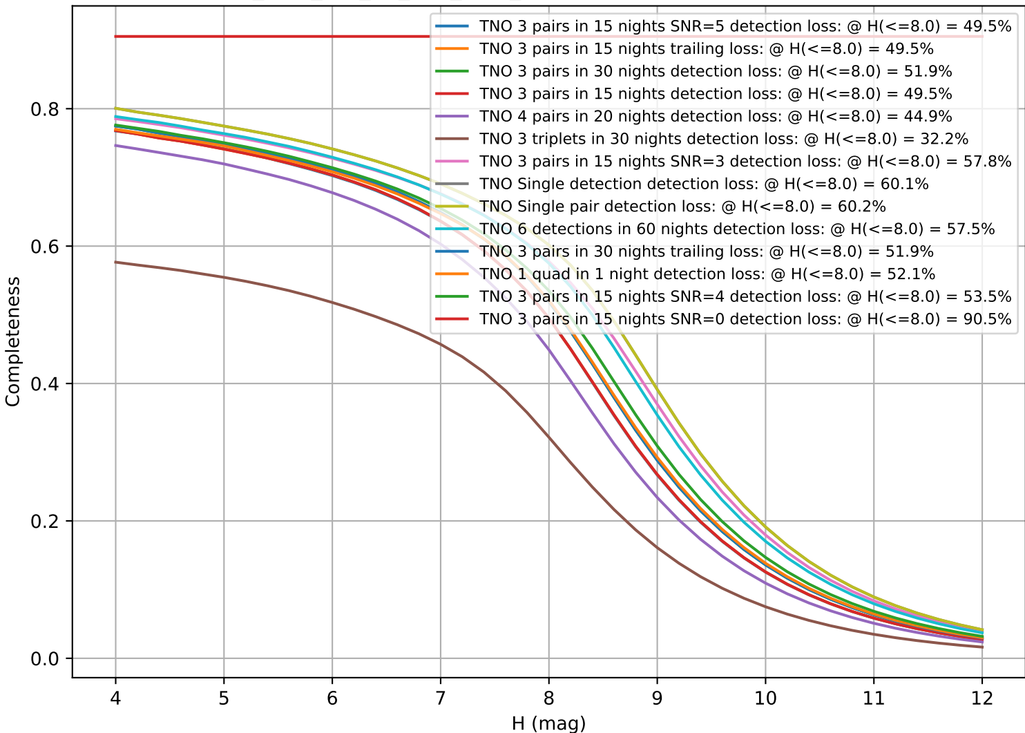
too_elab_r16_d2_griz_v3.4_10yrs: CumulativeCompleteness
