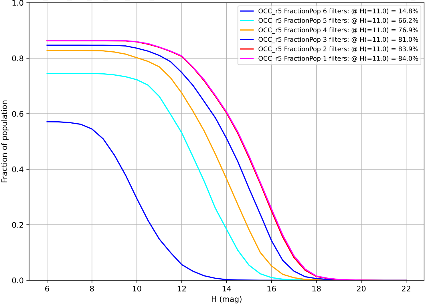
too_elab_r16_d2_griz_v3.4_10yrs: Fraction of population with colors in X filters OCC_r5
