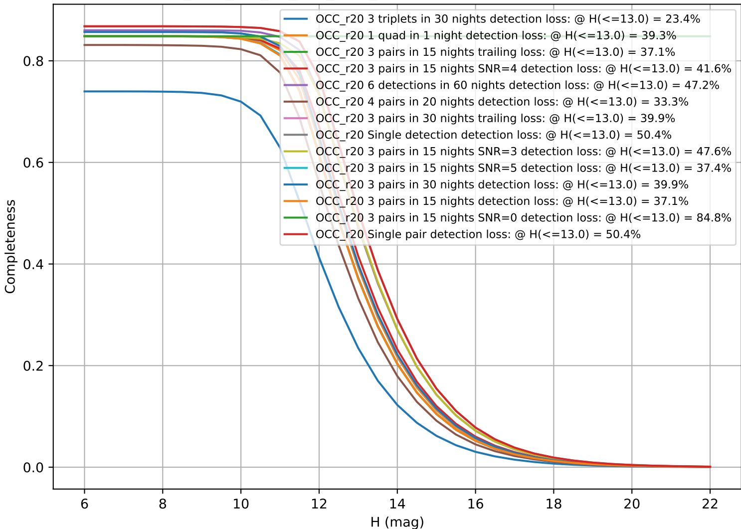
too_elab_r16_d2_griz_v3.4_10yrs: CumulativeCompleteness
