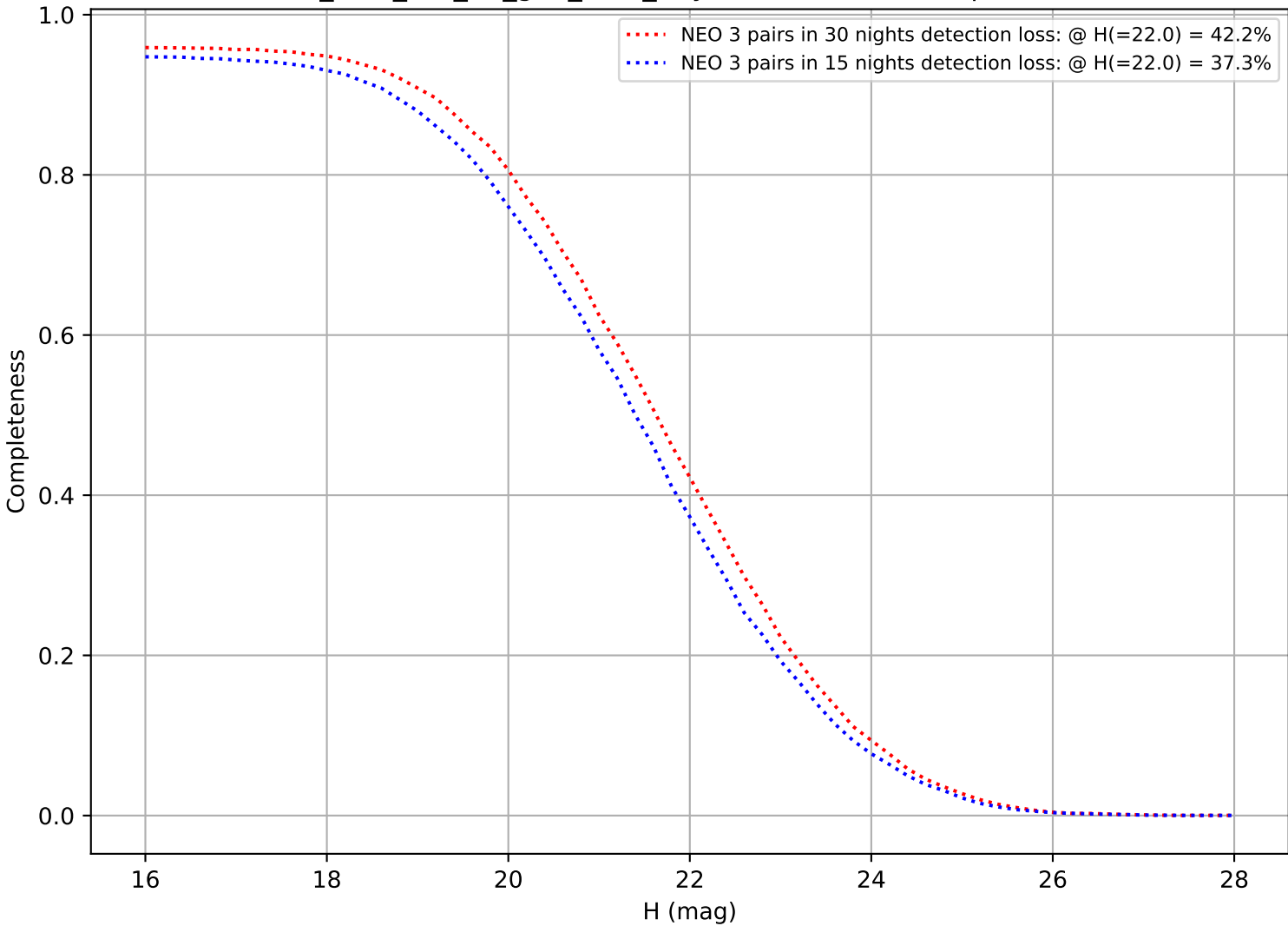
too_elab_r16_d2_griz_v3.4_10yrs: DifferentialCompleteness
