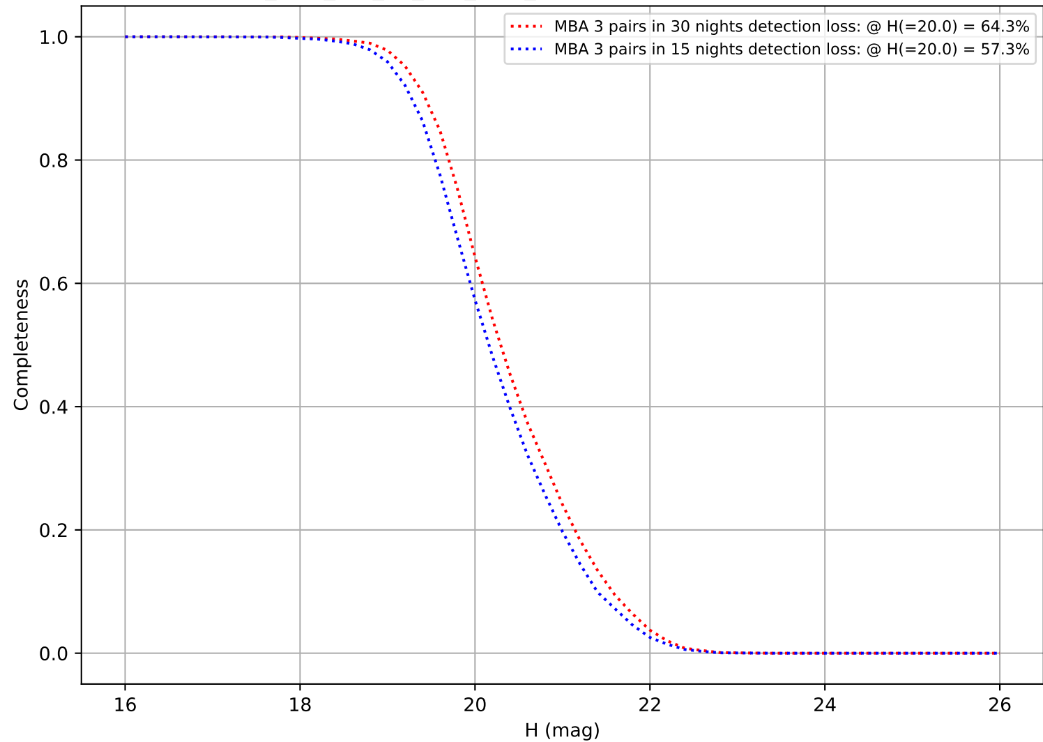
too_elab_r16_d2_griz_v3.4_10yrs: DifferentialCompleteness
