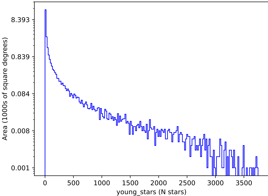
too_elab_r16_d2_griz_v3.4_10yrs : young_stars
