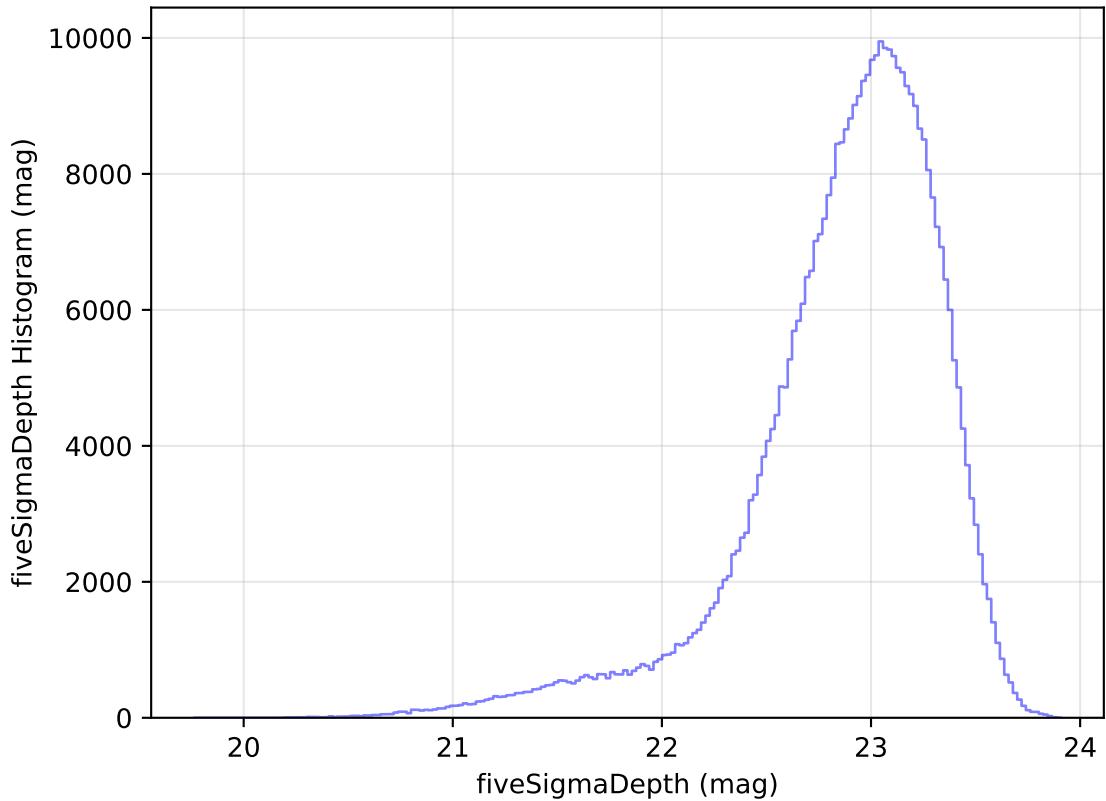
too_elab_r16_d2_griz_v3.4_10yrs z: fiveSigmaDepth Histogram
