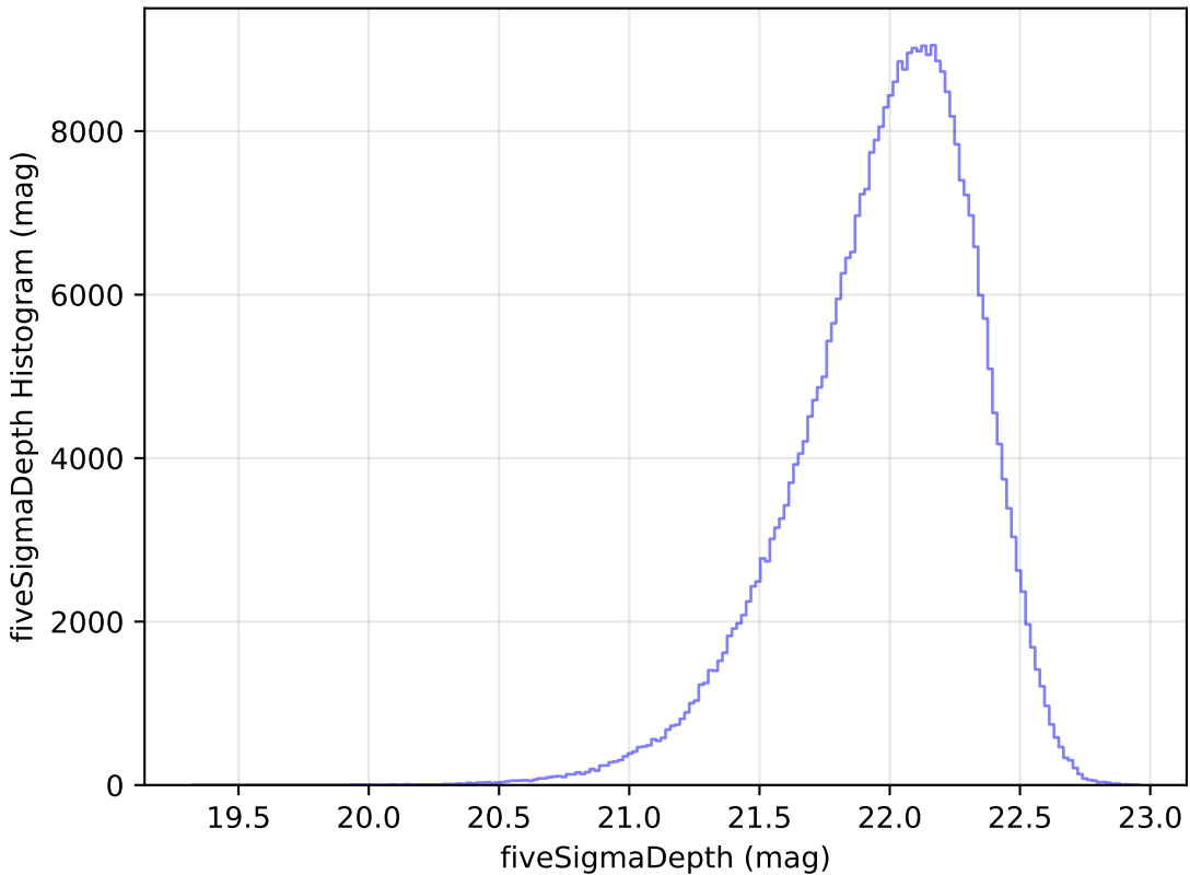
too_elab_r16_d2_griz_v3.4_10yrs y: fiveSigmaDepth Histogram
