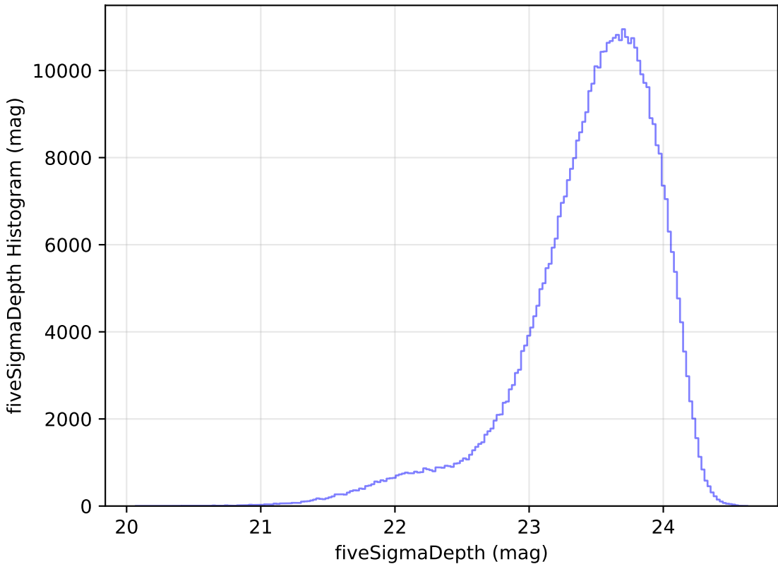
too_elab_r16_d2_griz_v3.4_10yrs i: fiveSigmaDepth Histogram
