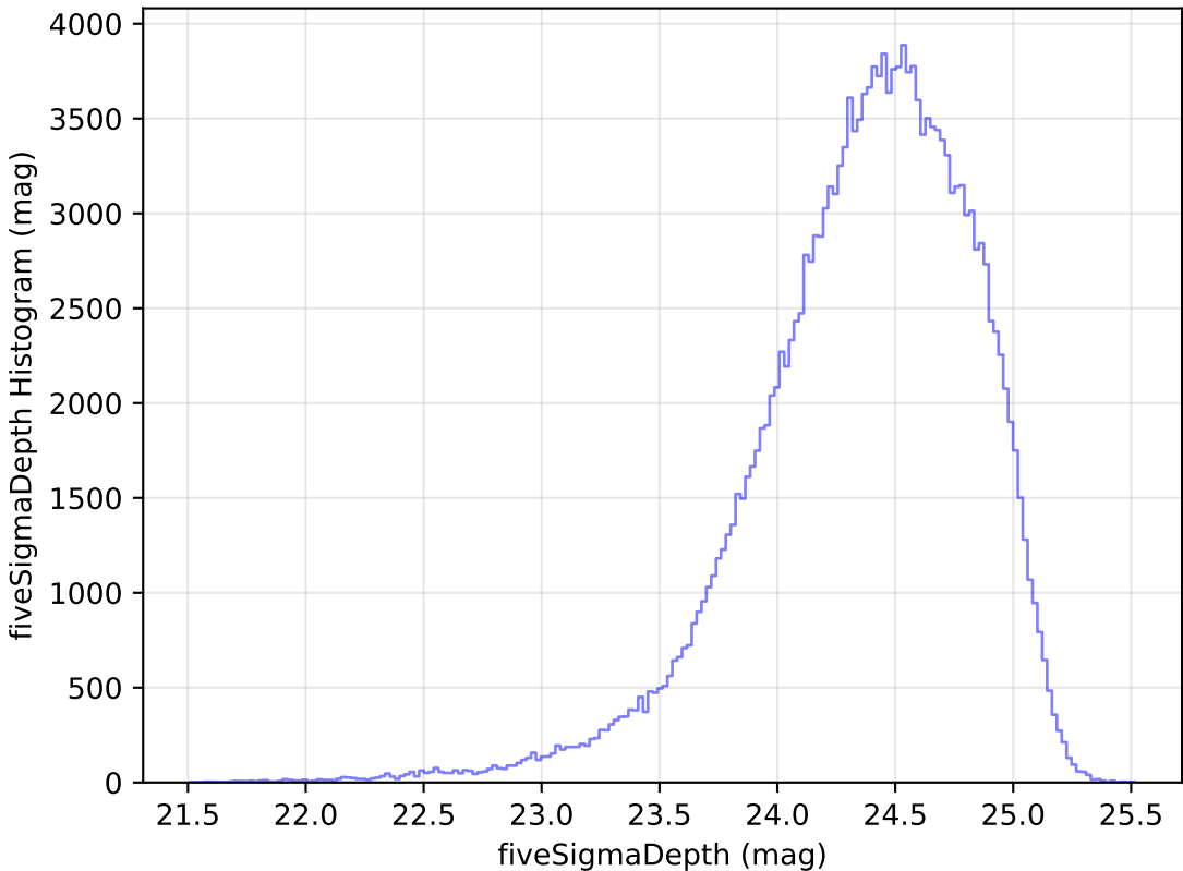
too_elab_r16_d2_griz_v3.4_10yrs g: fiveSigmaDepth Histogram
