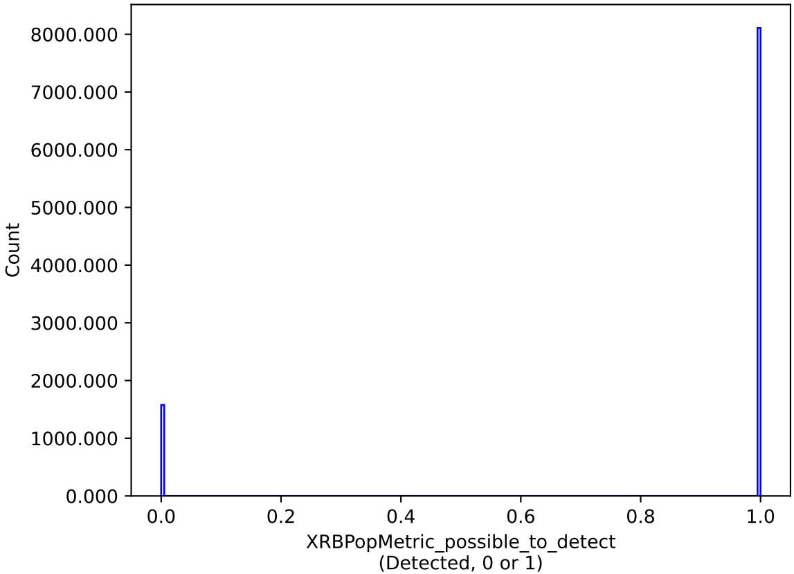
too_elab_r16_d2_griz_v3.4_10yrs : XRBPopMetric_possible_to_detect
