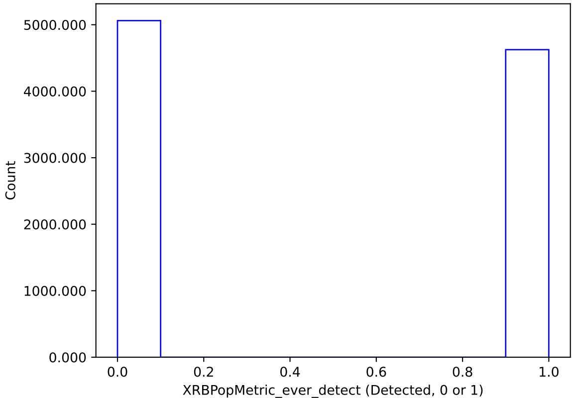
too_elab_r16_d2_griz_v3.4_10yrs : XRBPoMetric_ever_detect
