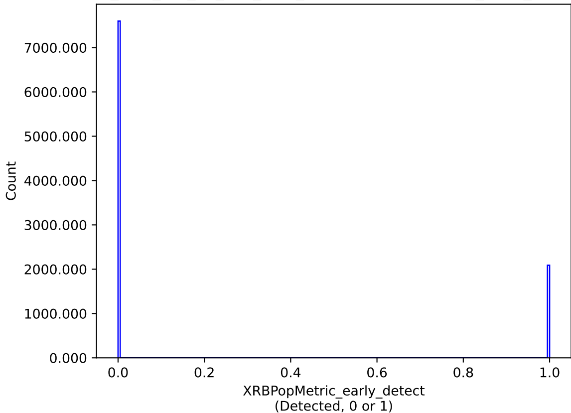
too_elab_r16_d2_griz_v3.4_10yrs : XRBPoMetric_early_detect
