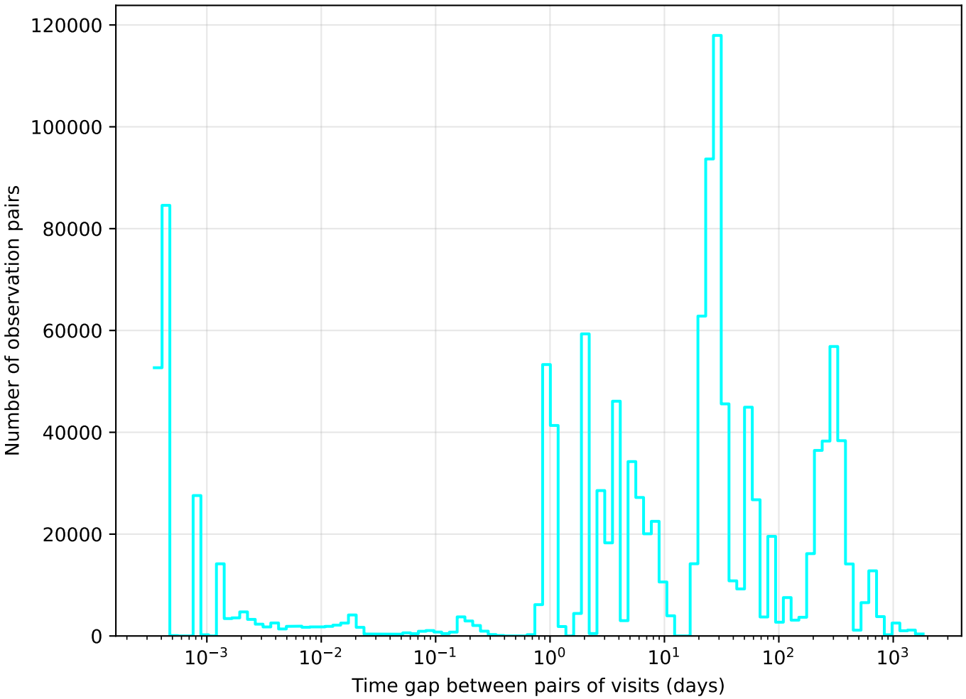
too_elab_r16_d2_griz_v3.4_10yrs u band: Tgaps observationStartMJD
