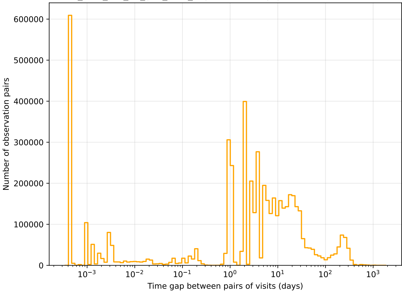
too_elab_r16_d2_griz_v3.4_10yrs r band: Tgaps observationStartMJD
