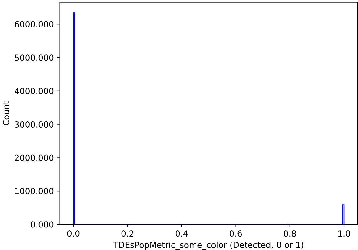
too_elab_r16_d2_griz_v3.4_10yrs : TDEsPopMetric_some_color
