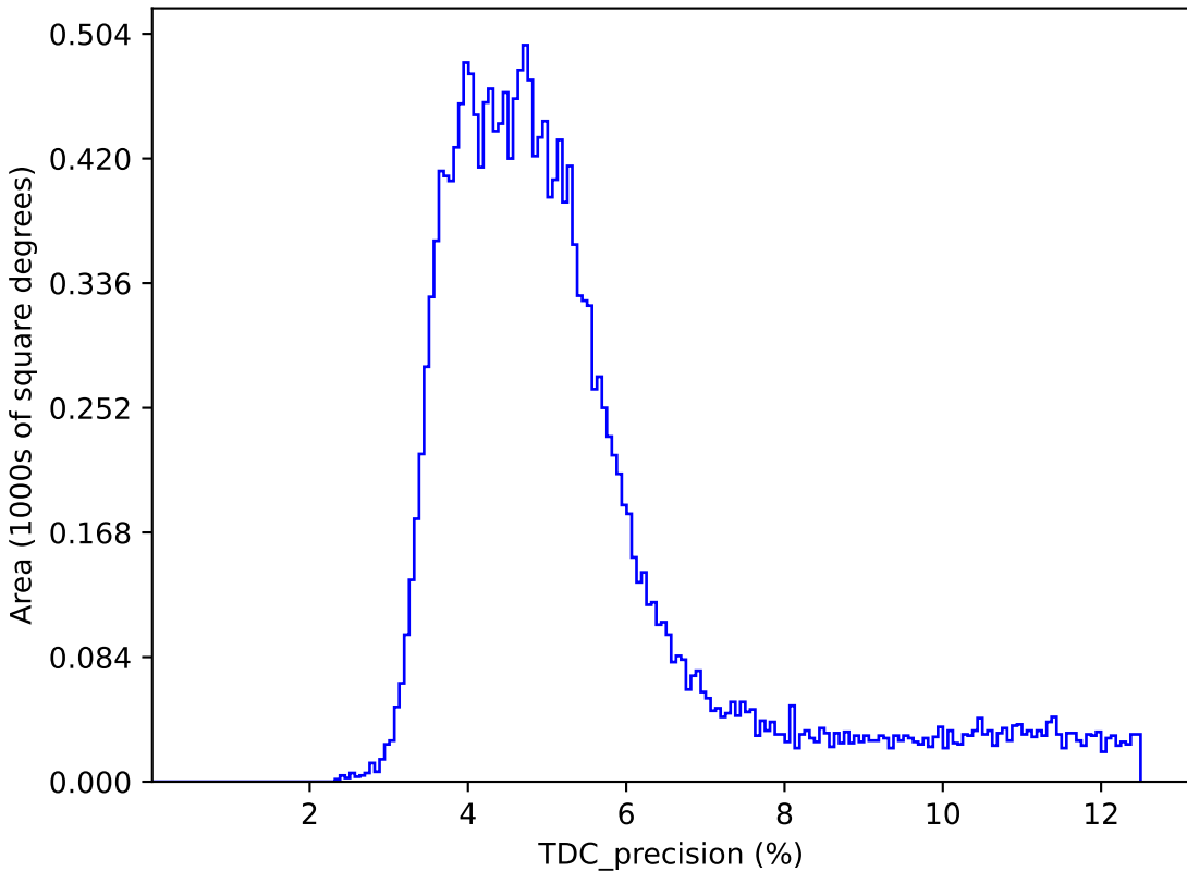
too_elab_r16_d2_griz_v3.4_10yrs : TDC_precision
