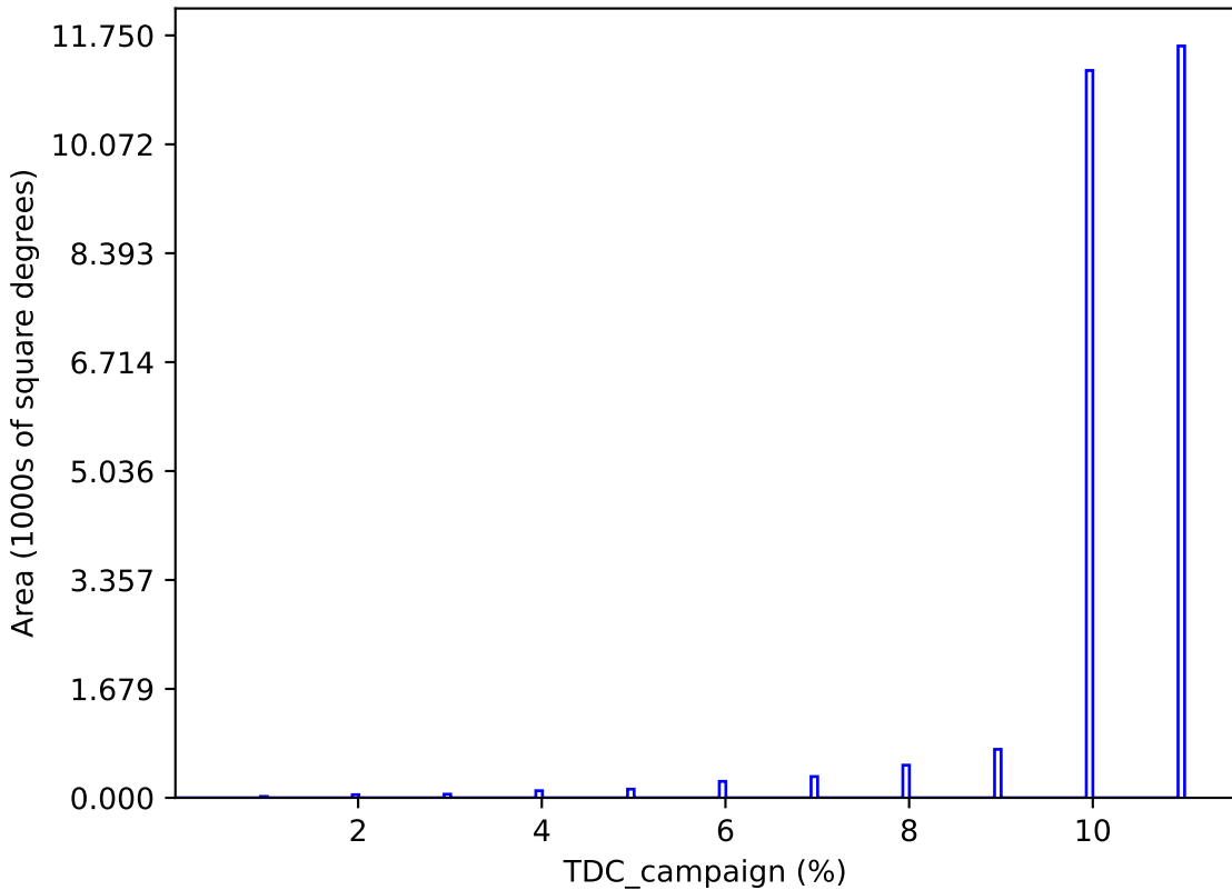
too_elab_r16_d2_griz_v3.4_10yrs : TDC_campaign
