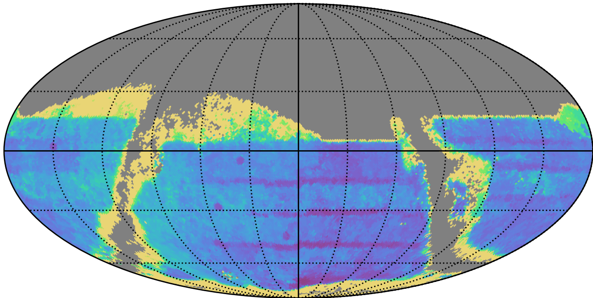
too_elab_r16_d2_griz_v3.4_10yrs : TDC_accuracy
