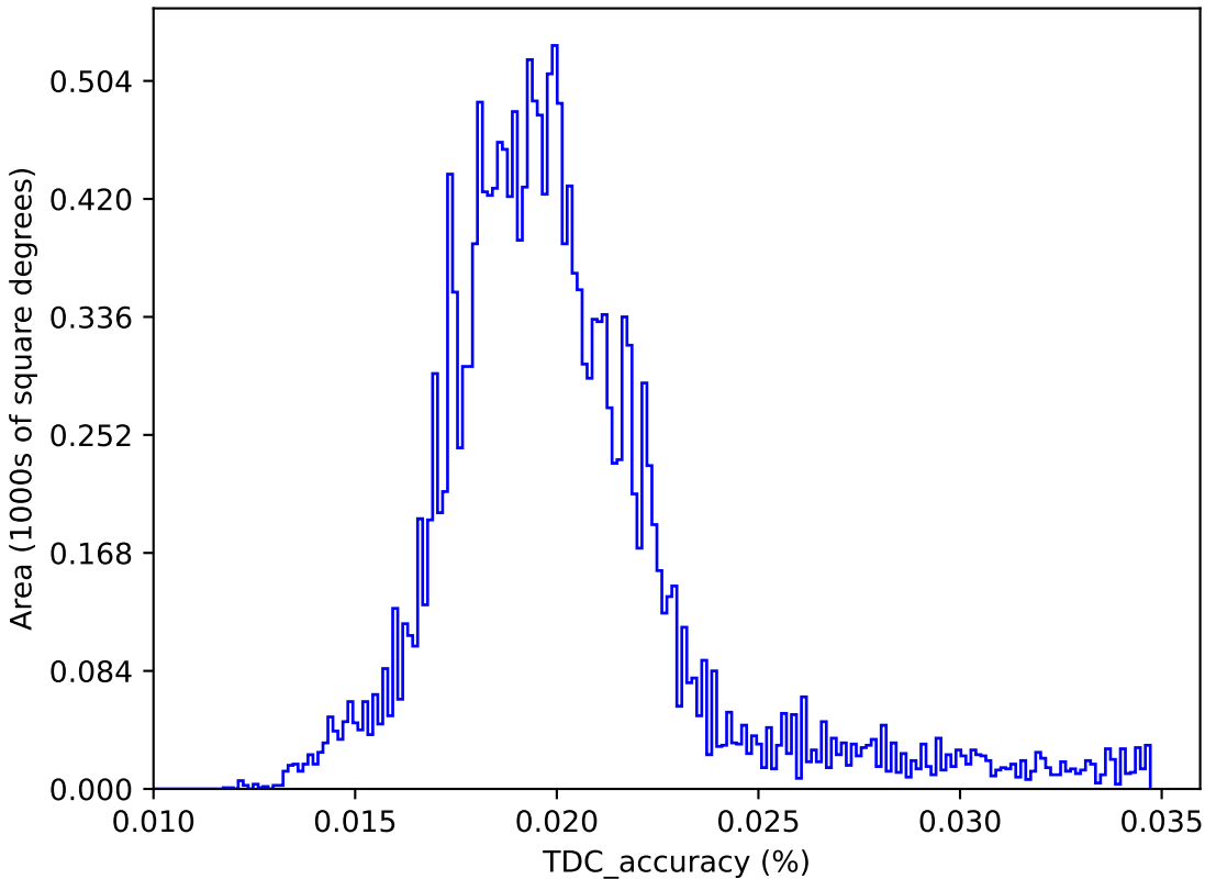
too_elab_r16_d2_griz_v3.4_10yrs : TDC_accuracy
