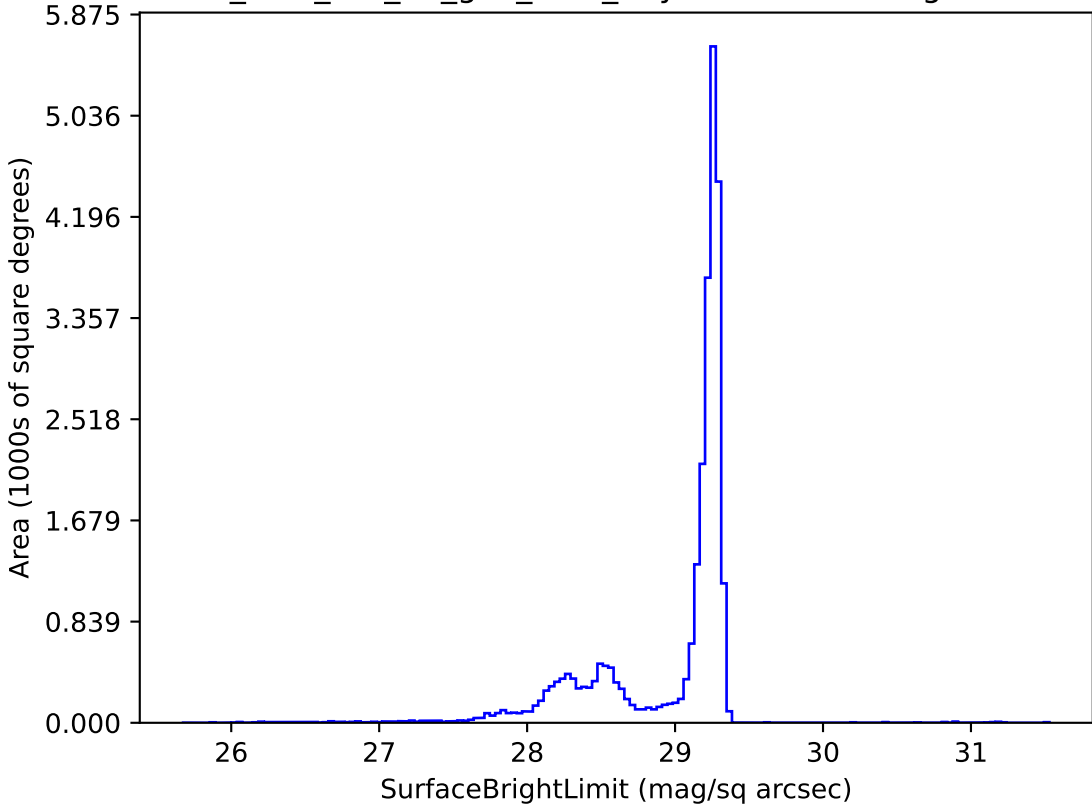
too_elab_r16_d2_griz_v3.4_10yrs z: SurfaceBrightLimit
