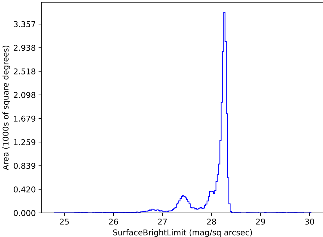
too_elab_r16_d2_griz_v3.4_10yrs y: SurfaceBrightLimit
