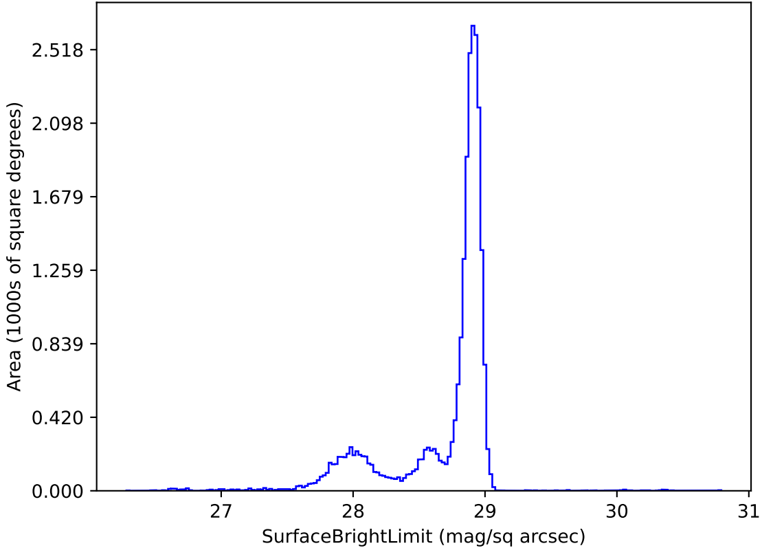
too_elab_r16_d2_griz_v3.4_10yrs u: SurfaceBrightLimit
