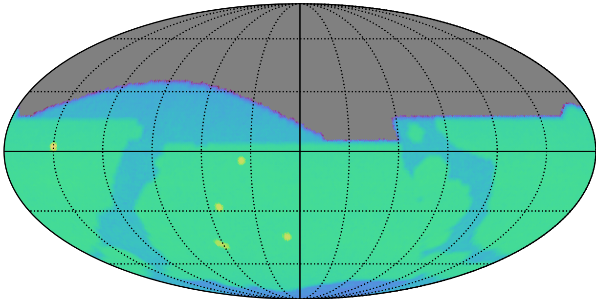
too_elab_r16_d2_griz_v3.4_10yrs i: SurfaceBrightLimit
