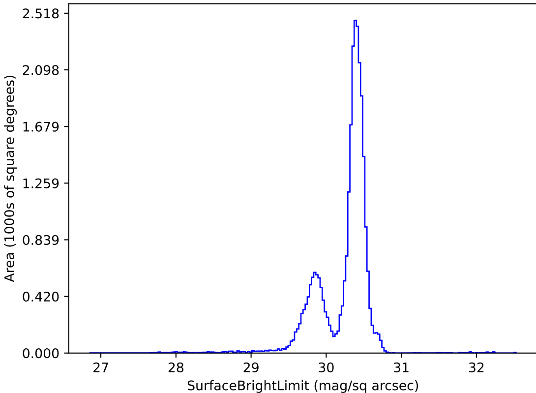
too_elab_r16_d2_griz_v3.4_10yrs g: SurfaceBrightLimit
