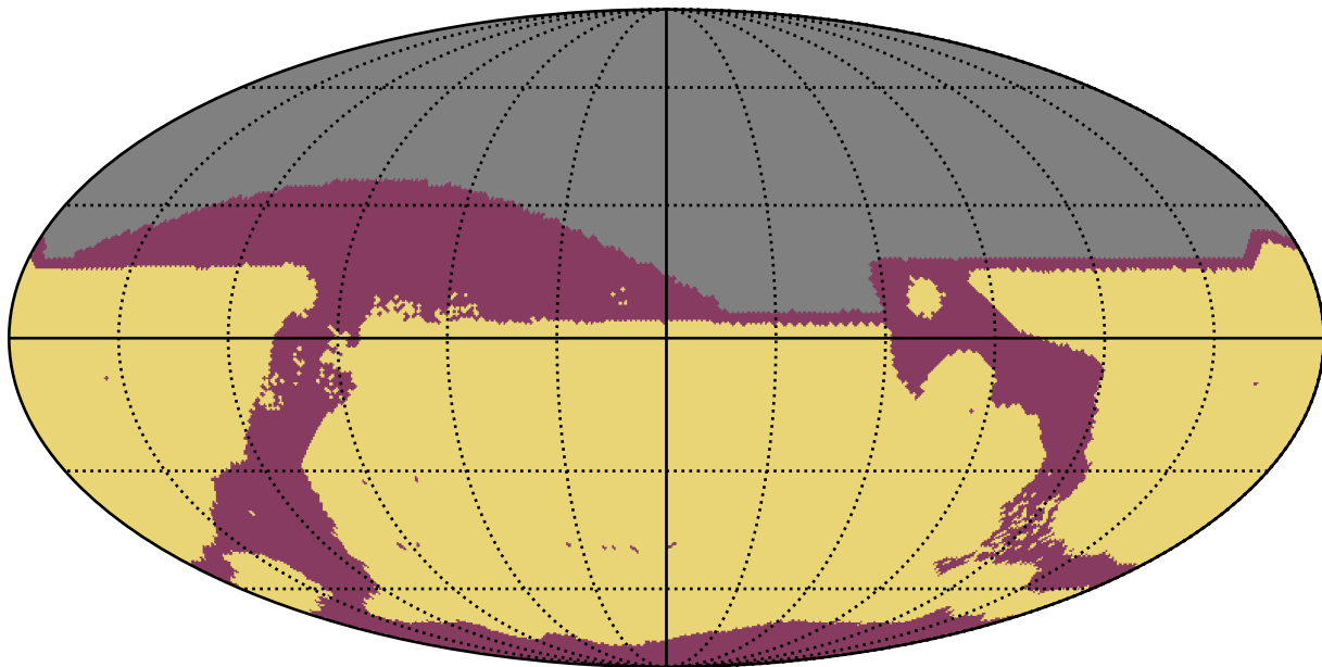
too_elab_r16_d2_griz_v3.4_10yrs : RapidRevisits
