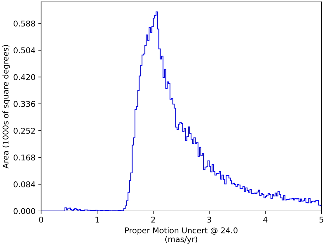
too_elab_r16_d2_griz_v3.4_10yrs : Proper Motion Uncert @ 24.0
