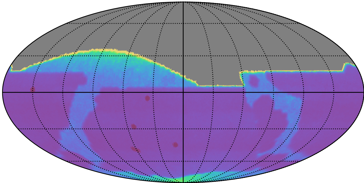
too_elab_r16_d2_griz_v3.4_10yrs : Proper Motion Uncert @ 20.5
