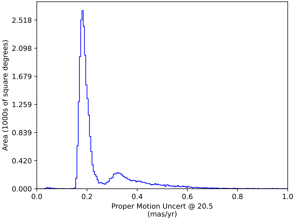
too_elab_r16_d2_griz_v3.4_10yrs : Proper Motion Uncert @ 20.5
