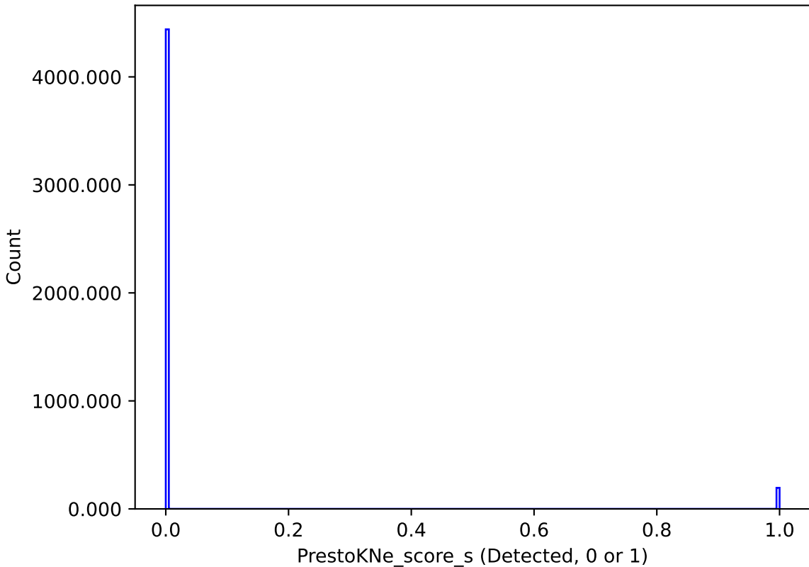
too_elab_r16_d2_griz_v3.4_10yrs : PrestoKNe_score_s
